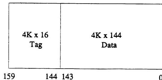
Figure 6-6: Level-2 Cache Organization
