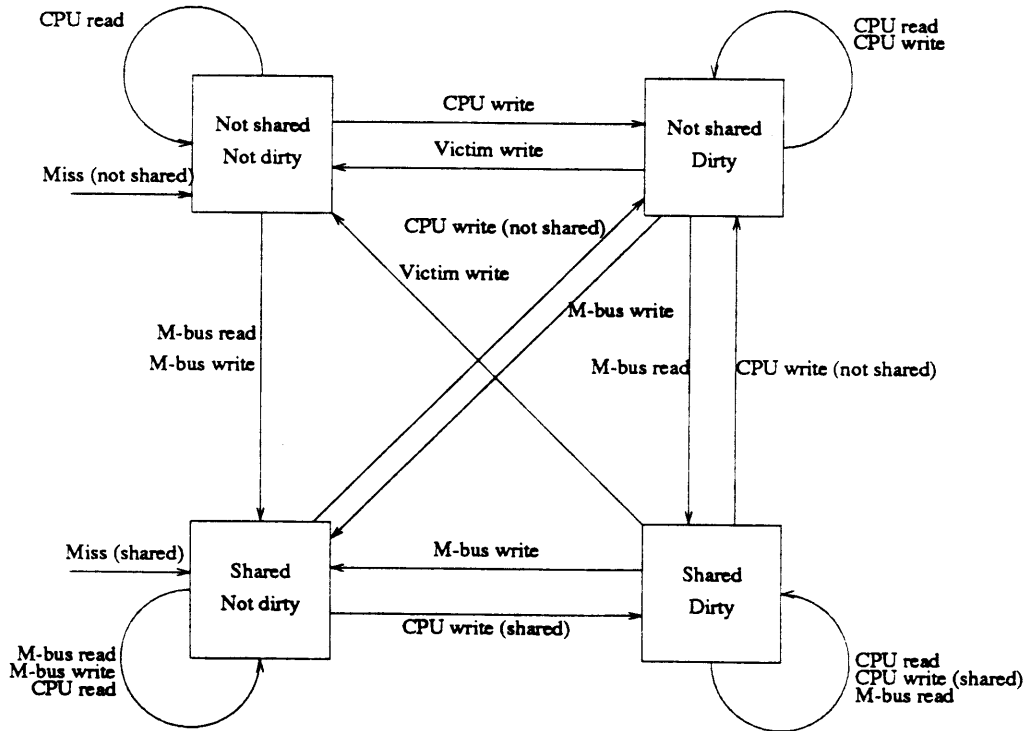
Figure 6-2: Snoopy Cache State Transitions
