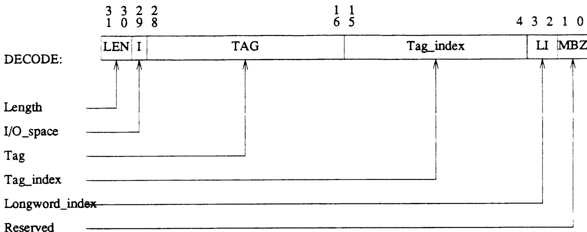
Figure 6-9: Level-2 Cache Address Decode
