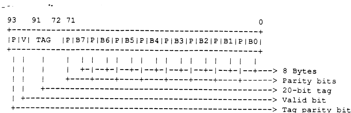
Figure 6-5: CVAX Level-1 Cache Line
